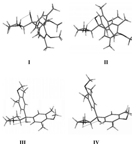
Figure 3. Calculated ammonium conformers of 2b (I–III) and 4a (II–IV).
