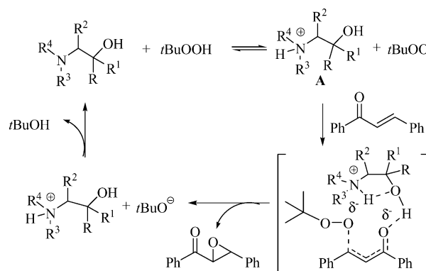
Figure 2. Proposed catalytic cycle for \beta -amino alcohols catalyzed epoxidation.
