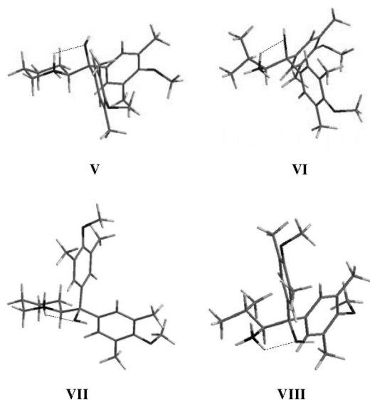
Figure 4. Calculated ammonium conformers of 5a (V–VII) and 12a (VI–VIII).
