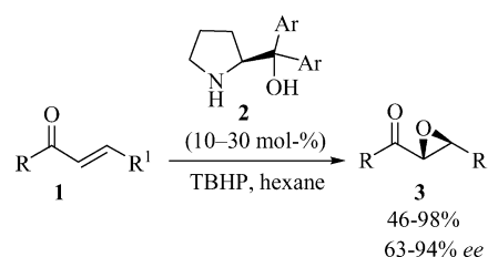
Scheme 1. Diaryl-2-pyrrolidinmethanol-catalyzed asymmetric epoxidations of \alpha,\beta -enones.
